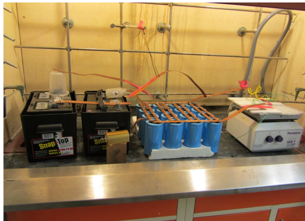
Figure 3 Step Stress Circuit
