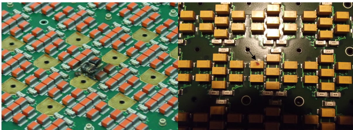
Figure 1 Damage comparison between MnO_2 (left) and polymer Tantalum Capacitor Failures
