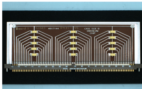
Figure 2 Typical Test Board
