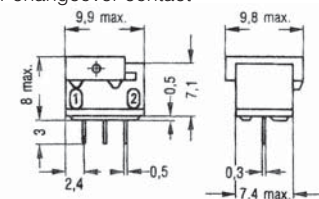
1 changeover contact
