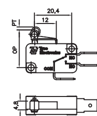
short roller
