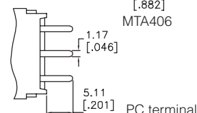
PC terminal
