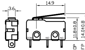
normal lever
