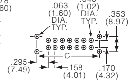
CONTACT ARRANGEMENT
