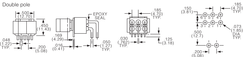
Double pole
