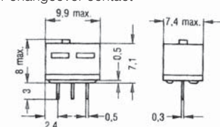
1 changeover contact
