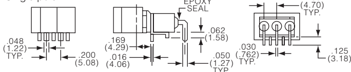
Single pole
