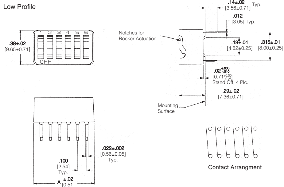
Low Profile
