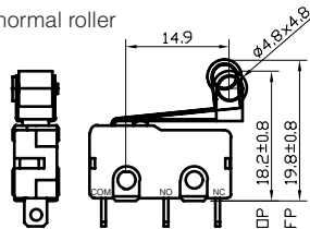
normal roller
