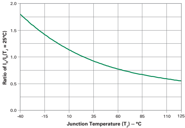
Figure 1: Normalized DC Holding Current vs. Junction Temperature
