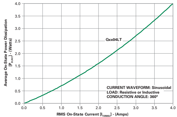
Figure 4: Power Dissipation vs. RMS On-State Current (Typical) (4A)
