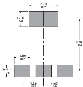
Dimensions in Millimeters (Inches)
