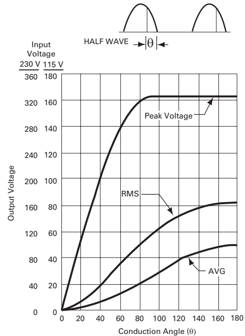
Figure AN1003.5 Output Voltage of Half-wave Phase
