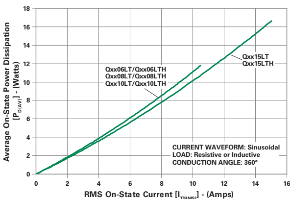
Figure 5: Power Dissipation vs. RMS On-State Current (Typical) (6A to 15A)
