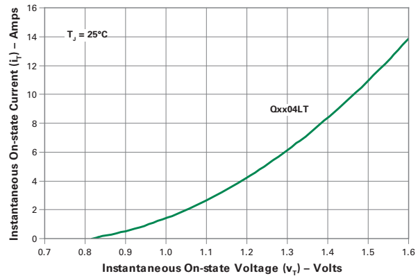
Figure 2: On-State Current vs. On-State Voltage (Typical) (4A)
